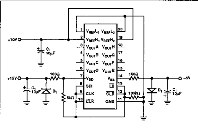
BURN-IN CIRCUIT
