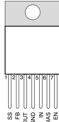
KTW Package 7-Pin DDPK/TO-263 Top View
