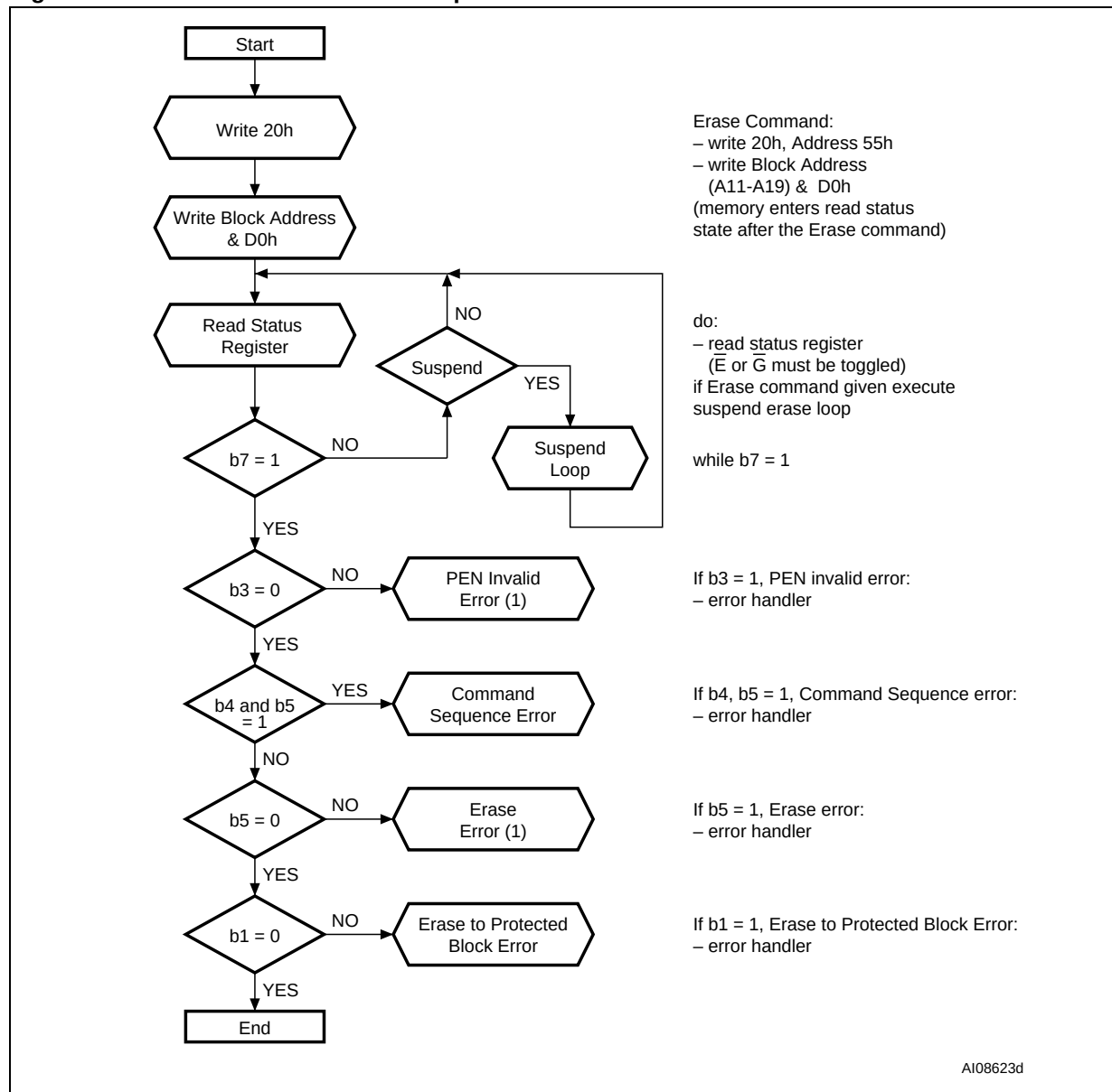
Figure 26. Block Erase flowchart and pseudo code
