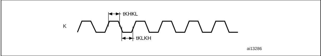
Figure 20. Clock input AC waveform
