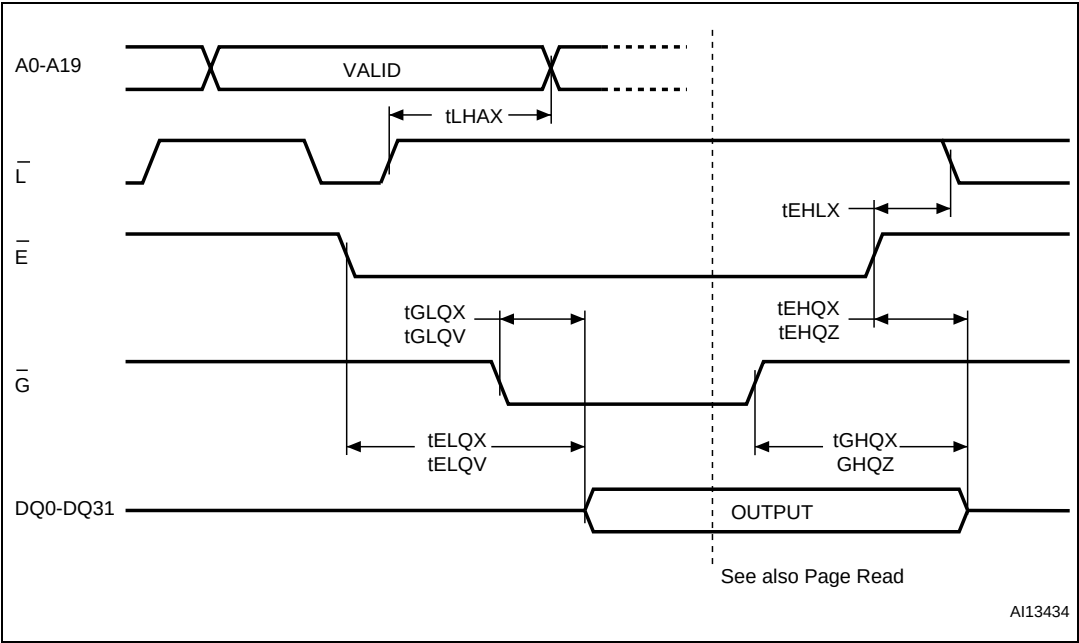
Figure 9. Asynchronous Chip Enable controlled bus Read AC waveforms
