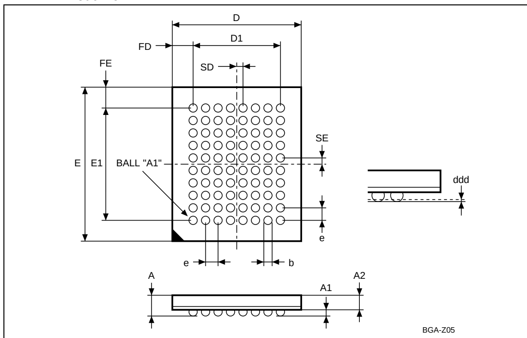
Figure 22. LBGA80 10 × 12mm - 8 × 10 ball array, 1mm pitch, bottom view package outline
