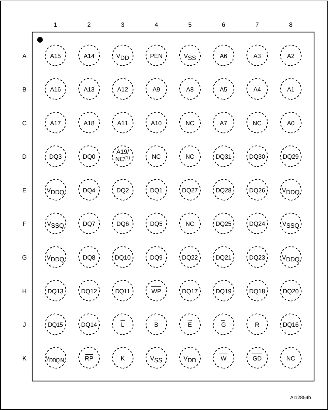
Figure 2. LPGA connections (top view through package)
