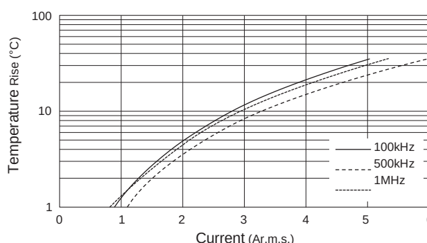
Ripple Current
