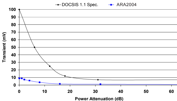
Figure 13: Transients vs Attenuation P_{OUT} = 55\text{dBmV} at 0dB attenuation
