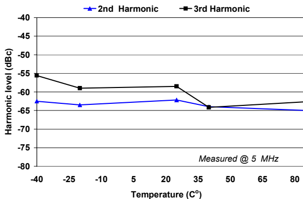
Figure 11: Harmonic Distortion vs Temperature P_{OUT} = 58\text{dBmV}
