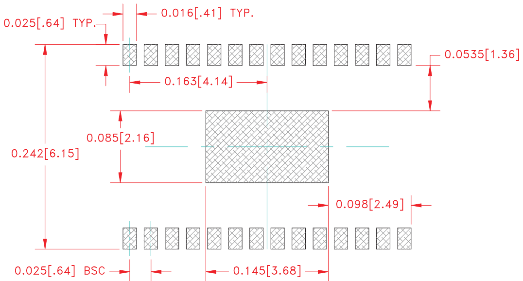
Figure 19: Solder Mask Outline
