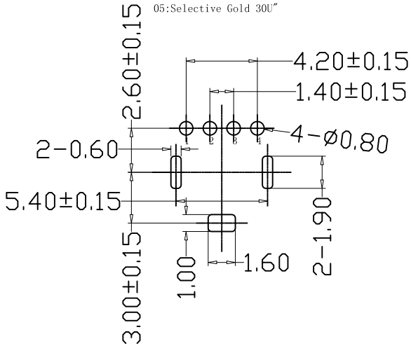
RECOMMENDED PCB LAYOUT GENERAL TOLERANCES: ±0.05
