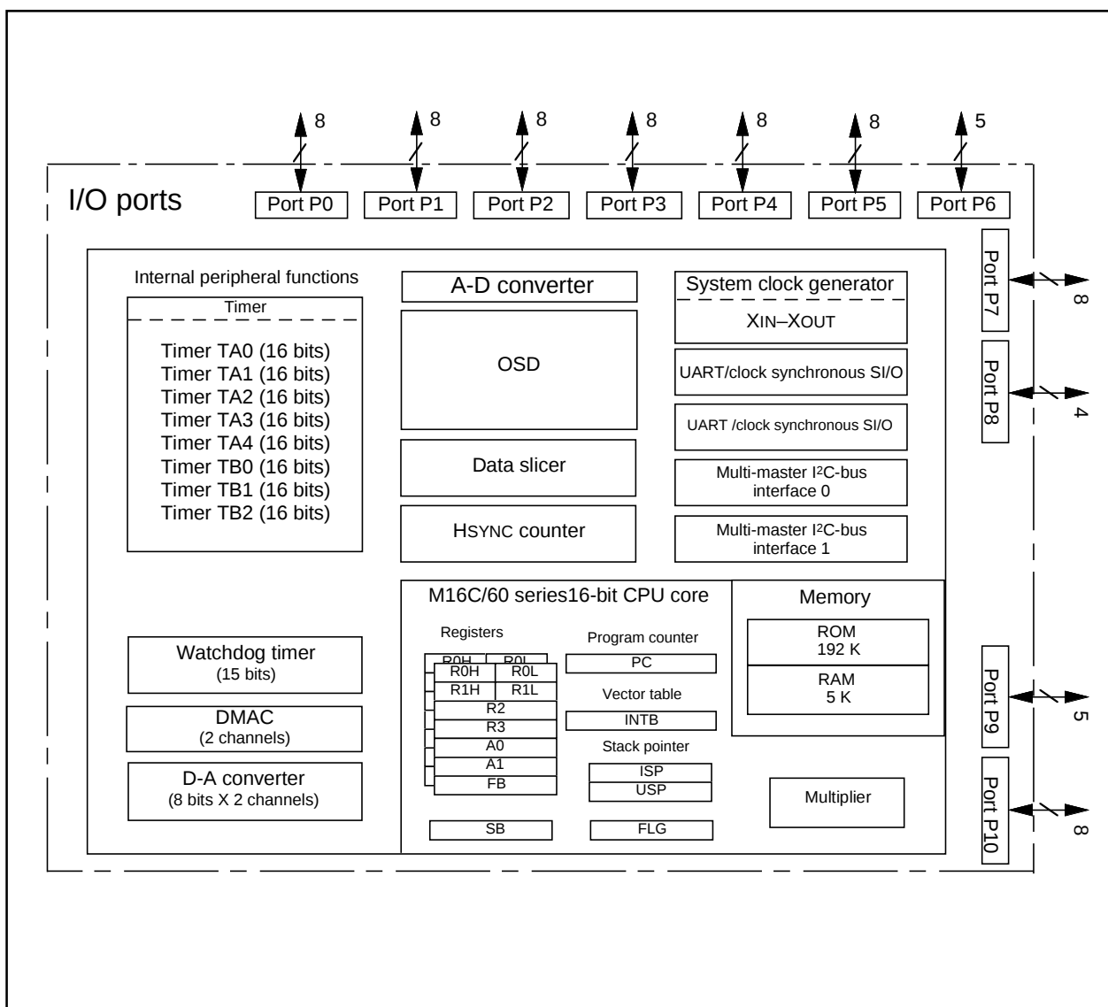
Figure 1.4.1 Block diagram
