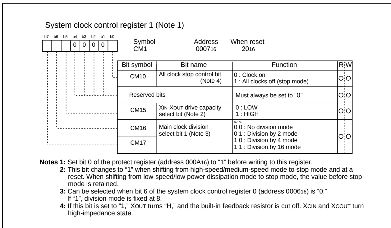
Figure 2.5.6 System clock control register 1
