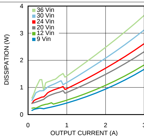
Figure 2. Dissipation 6-V Output at 25°C Ambient
