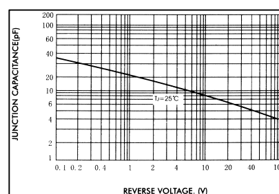
FIG.5-TYPICAL JUNCTION CAPACITANCE
