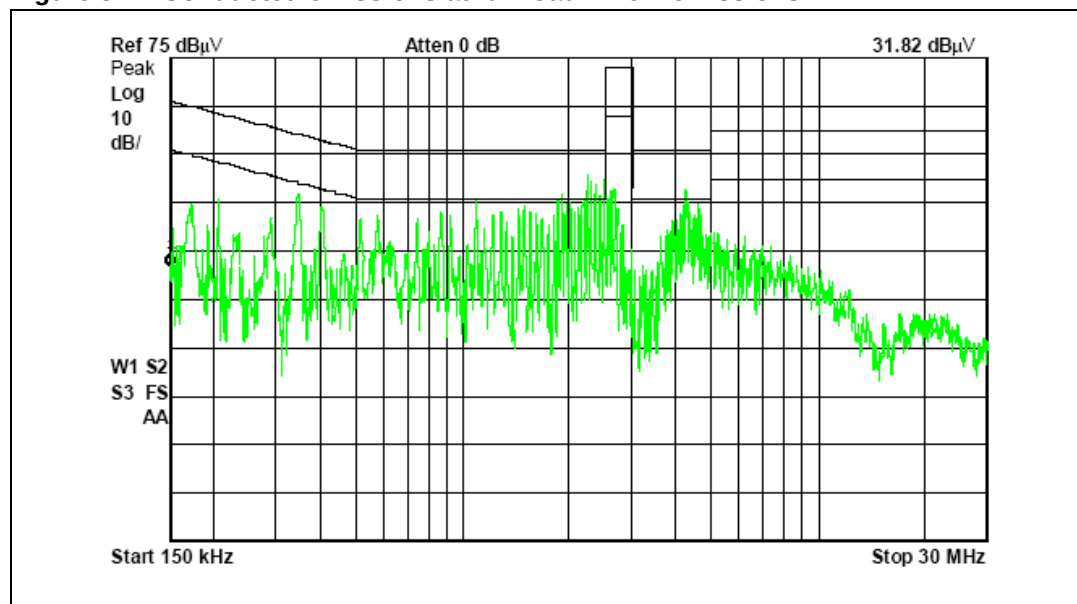
Figure 31. Conducted emissions at full load: line 1 emissions
