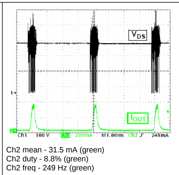
Figure 22. Drain voltage V_{DS} and output current I_{OUT} at 10% dimming: 8 LEDs
