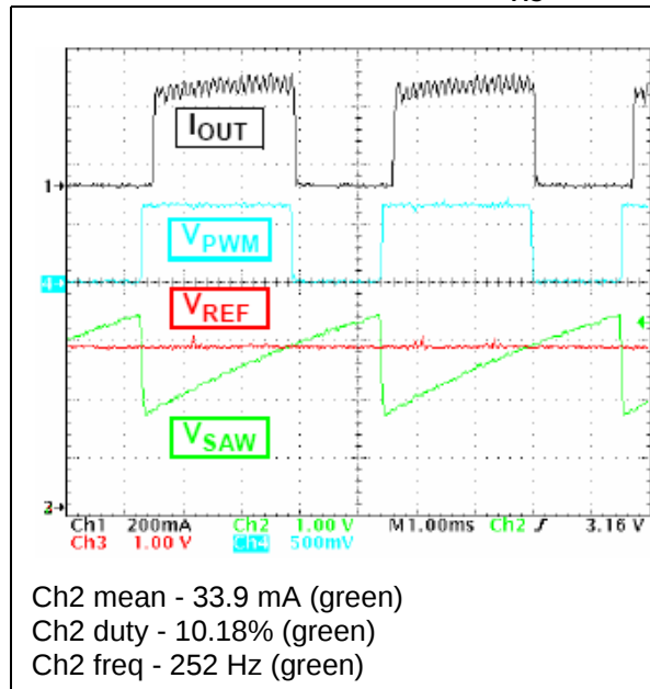
Figure 23. Control signals at 230 V AC : 1 LED
