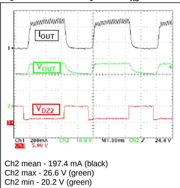
Figure 26. Control stage at 230 V AC : 8 LEDs
