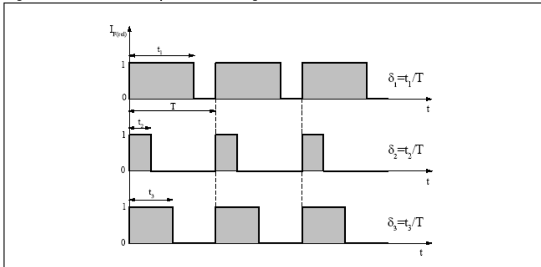
Figure 6. PWM technique for dimming
