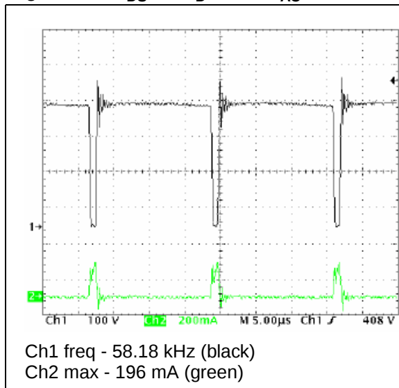
Figure 13. V DS and I D at 230 V AC : 1 LED
