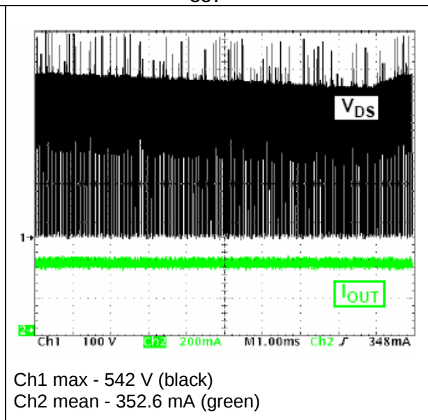
Figure 18. Drain voltage V DS and output current I OUT : 8 LEDs
