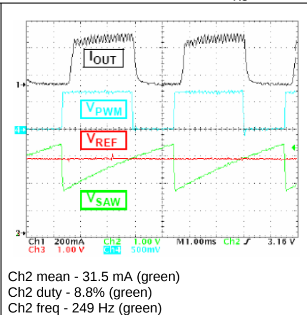
Figure 24. Control signals at 230 V AC : 8 LEDs
