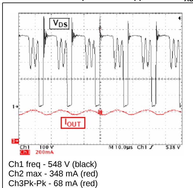
Figure 15. Typical waveforms: drain voltage and output current ripple at 230 V AC
