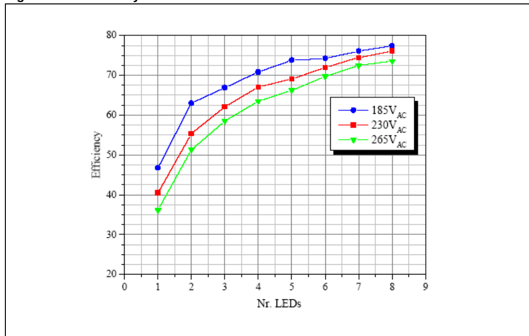
Figure 29. Efficiency
