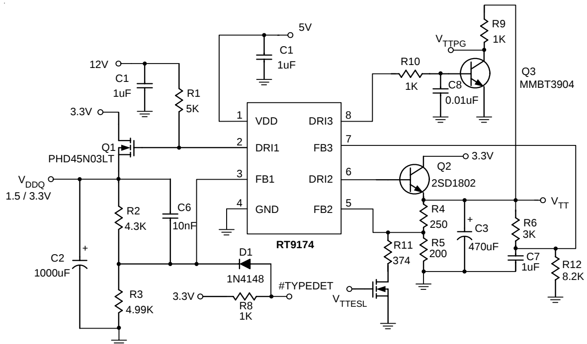
Figure 2. Dual LDOs with V_{TTPG} for VRM 8.5 Application
