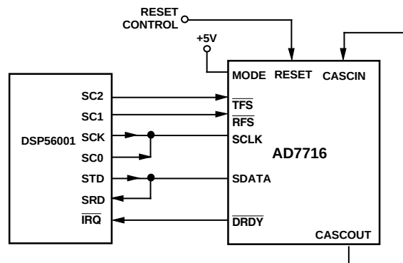
Figure 10. DSP56001 Interface
