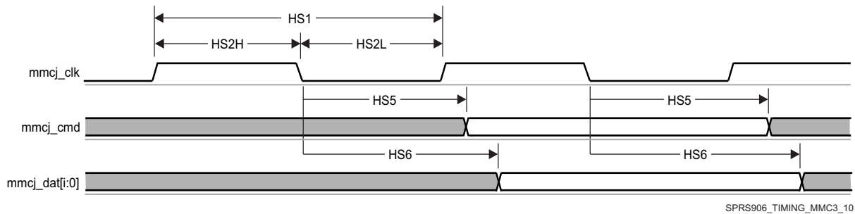
图 7-84. MMC/SD/SDIOj in - High Speed Signaling - Transmitter Mode
