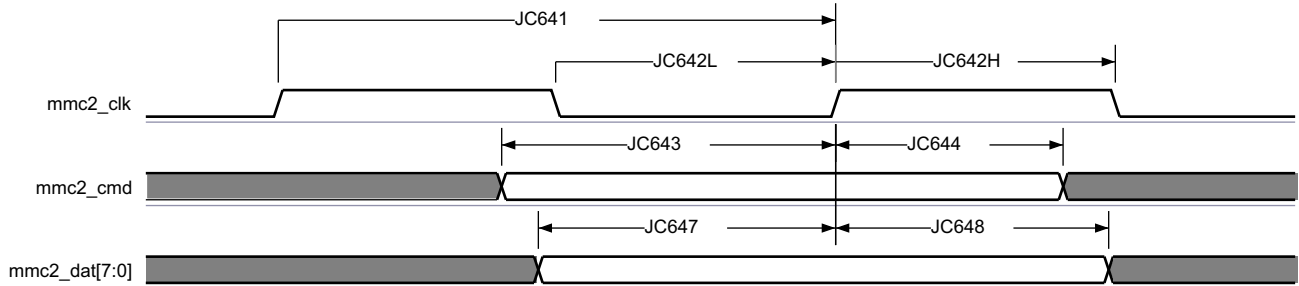
图 7-76. MMC/SD/SDIO in - High Speed JC64 - Receiver Mode
