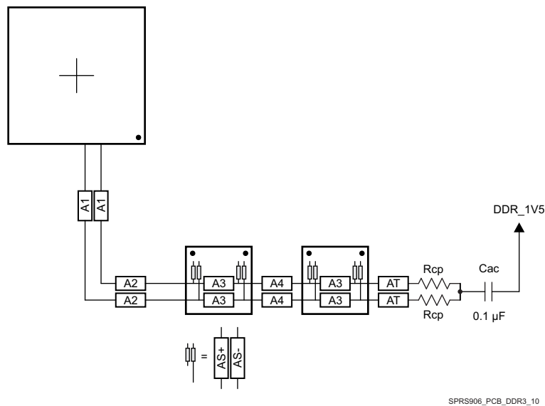
图 8-10. CK Routing for Four Mirrored DDR3 Devices
