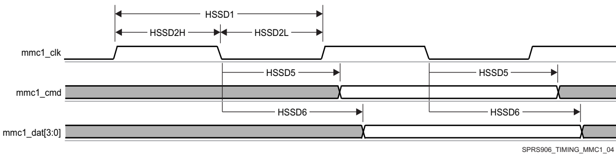
图 7-63. MMC/SD/SDIO in - High Speed - Transmitter Mode
