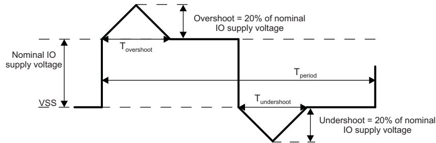
图 5-1. T_{\text{overshoot}} + T_{\text{undershoot}} < 20\% \text{ of } T_{\text{period}}
