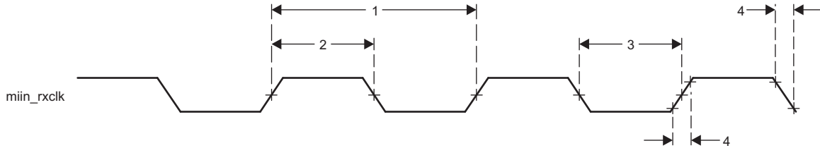
图 7-51. Clock Timing (GMAC Receive) - MII operation
