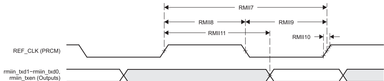
图 7-57. GMAC Transmit Interface Timing RMIIIn Operation
