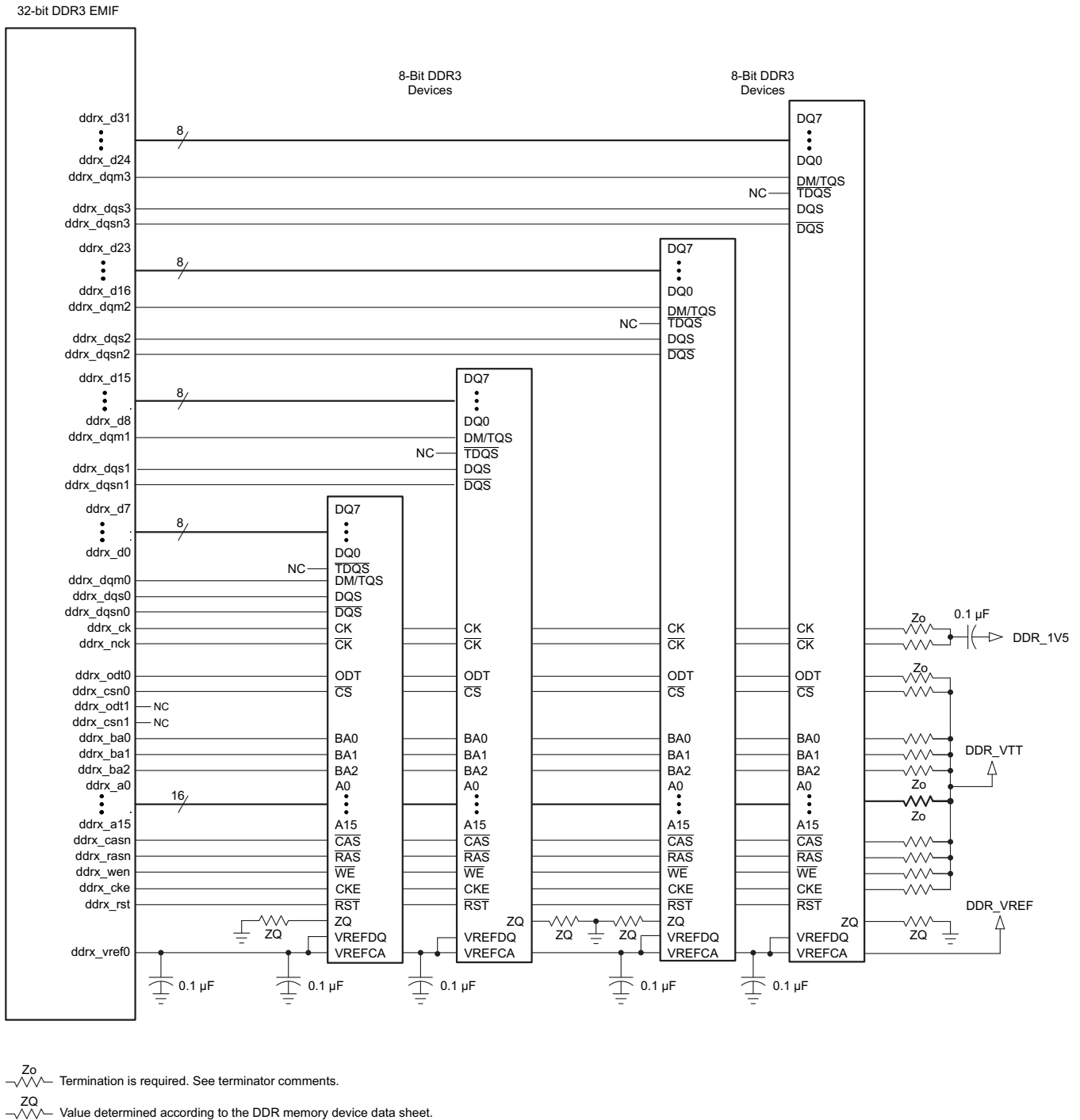
图 8-3. 32-Bit, One-Bank DDR3 Interface Schematic Using Four 8-Bit DDR3 Devices
