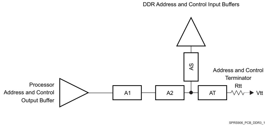
图 8-19. ADDR_CTRL Topology for One DDR3 Device
