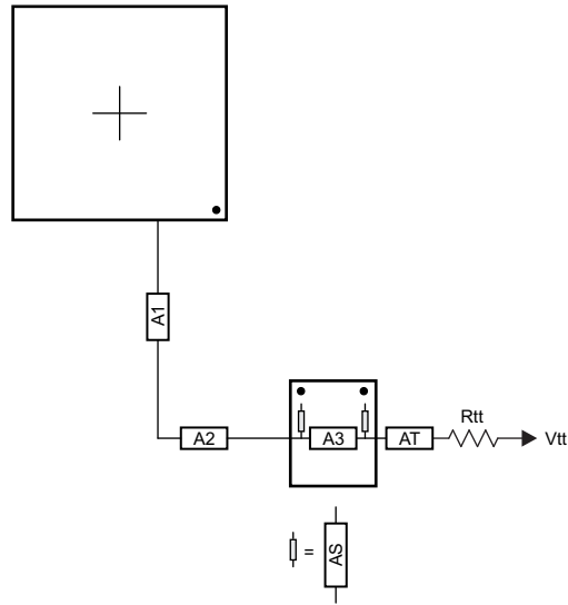
图 8-17. ADDR_CTRL Routing for Two Mirrored DDR3 Devices
