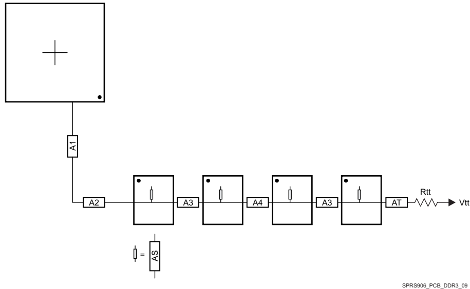
图 8-9. ADDR_CTRL Routing for Four Single-Side DDR3 Devices
