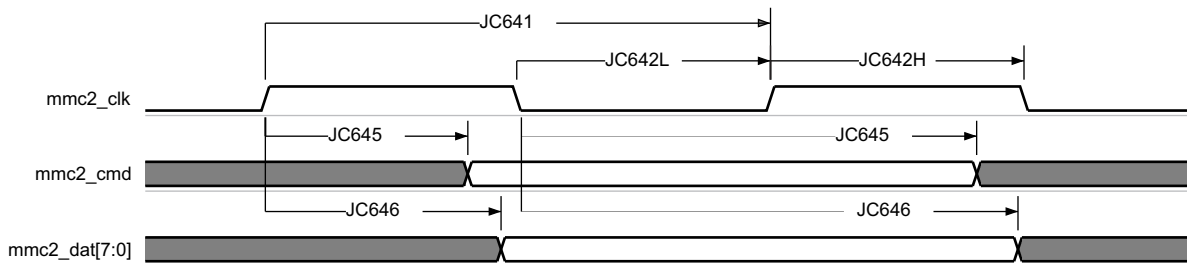
图 7-77. MMC/SD/SDIO in - High Speed JC64 - Transmitter Mode
