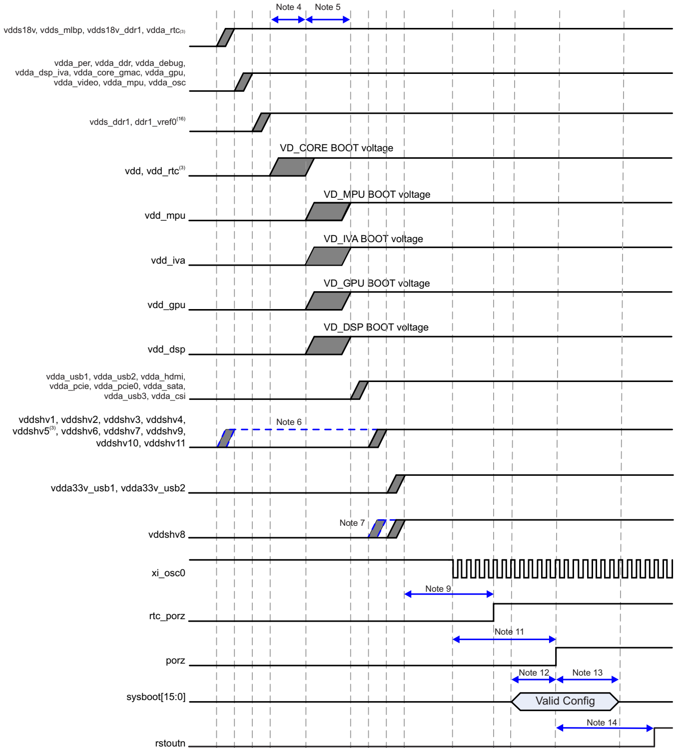
图 5-2. Power-Up Sequencing
