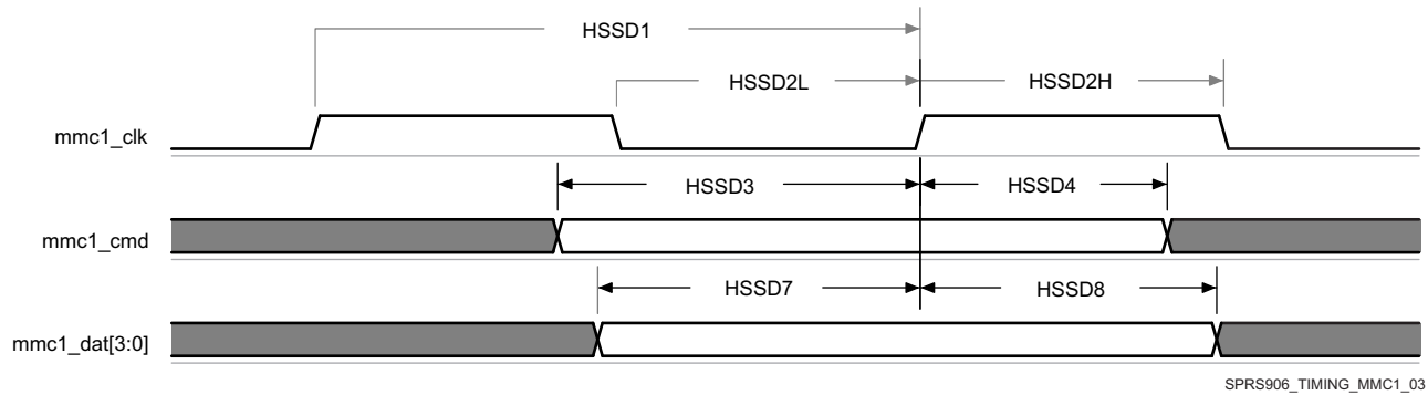
图 7-62. MMC/SD/SDIO in - High Speed - Receiver Mode
