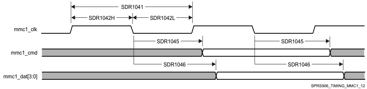
图 7-71. MMC/SD/SDIO in - High Speed SDR104 - Transmitter Mode
