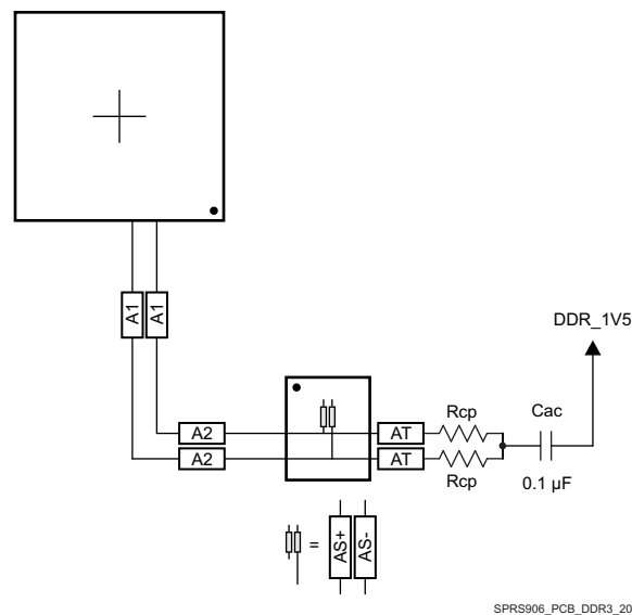
图 8-20. CK Routing for One DDR3 Device
