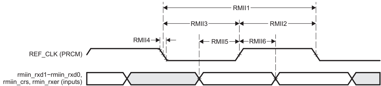
图 7-56. GMAC Receive Interface Timing RMIIIn operation
