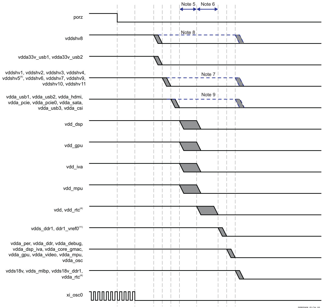
图 5-3. Power-Down Sequencing (10)(12)
