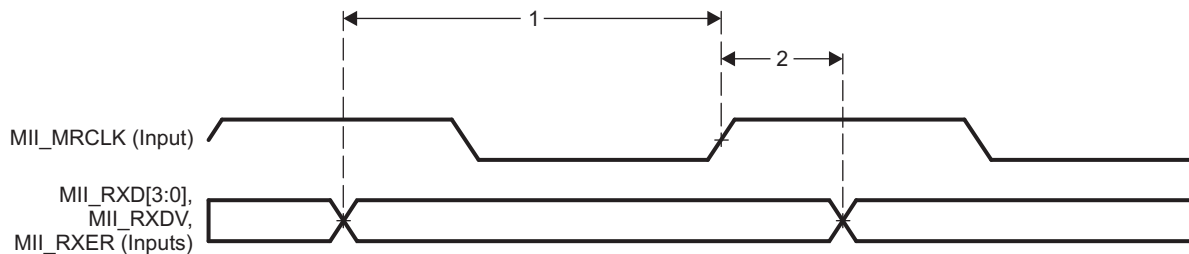
图 7-109. PRU-ICSS MII_RXD[3:0], MII_RXDV, and MII_RXER Timing
