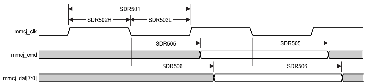
图 7-90. MMC/SD/SDIOj in - High Speed SDR50 - Transmitter Mode
