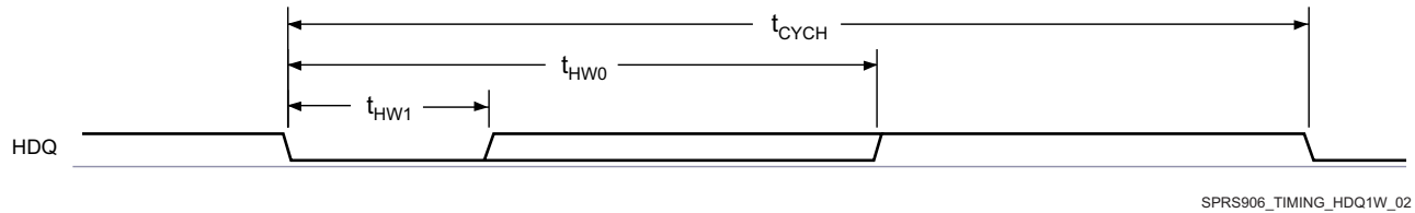
图 7-26. Device HDQ Interface Bit Read Timing (Data)
