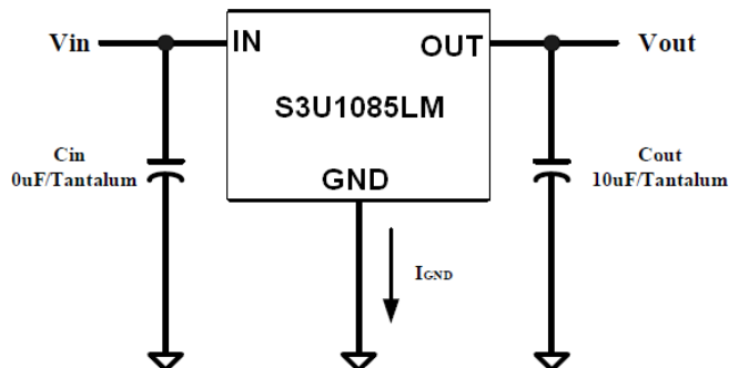
Figure2. Fixed Voltage Regulator
