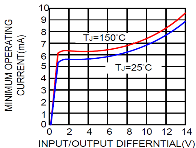
Minimum Operating Current
