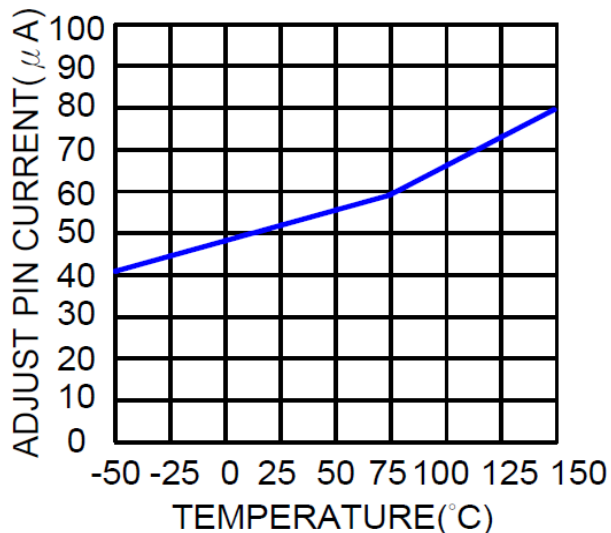
Adjust Pin Current
