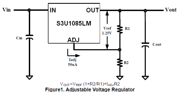
Figure1. Adjustable Voltage Regulator
