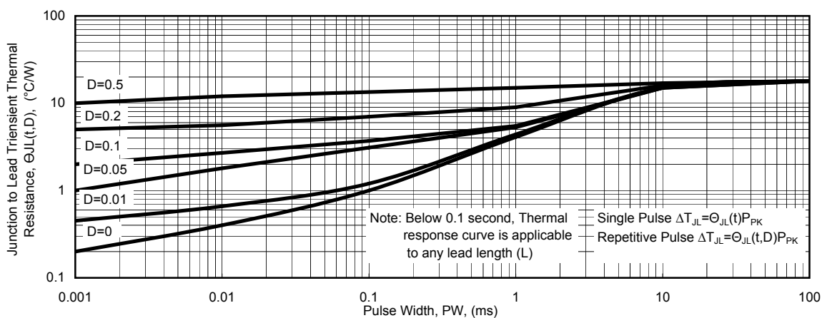
Fig. 5 - Typical Thermal Response L, Lead Length=3/8inch
