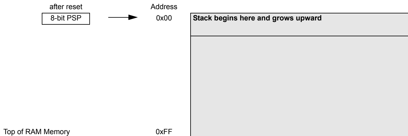
Figure 14-2. Data Memory Organization
