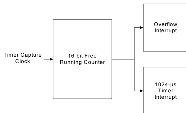
Figure 20-1. 16-bit Free Running Counter Block Diagram
