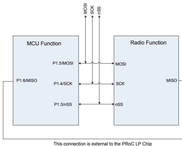
Figure 9-2. 4-Wire SPI Mode
