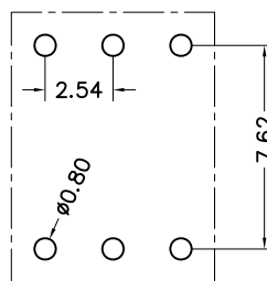
P. C. B LAYOUT
