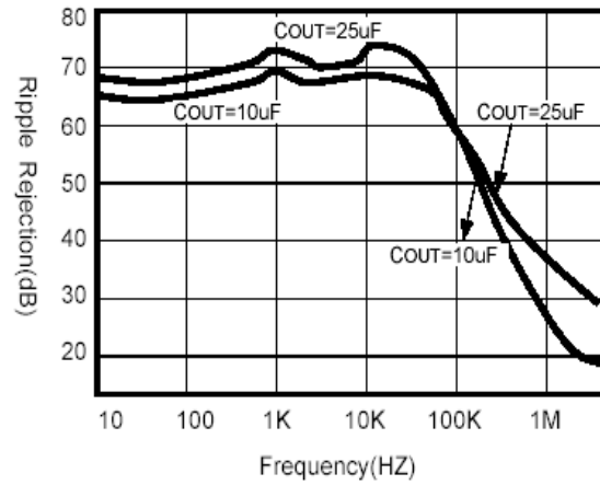
Ripple Rejection(with C_{adj} 25 \mu F)
