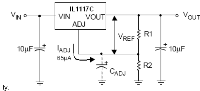
Figure 4. Basic Adjustable Regulator
