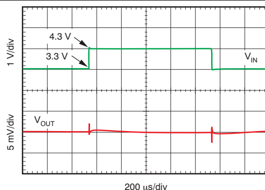
Figure 29. Line Transient Response V_{OUT} = 1.8 V , I_{OUT} = 500 mA
