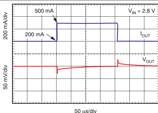
Figure 28. Load Transient Response 200 mA to 500 mA, C_{OUT} = 1 \mu F
