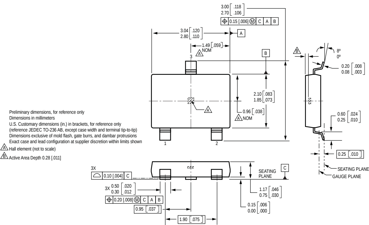
Pin-out Drawings
