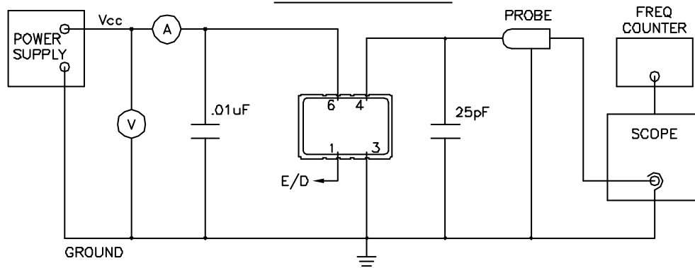
TEST CIRCUIT
