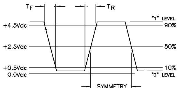
OUTPUT WAVEFORM
