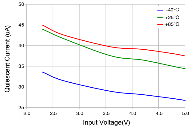
Figure 20. Quiescent Current
