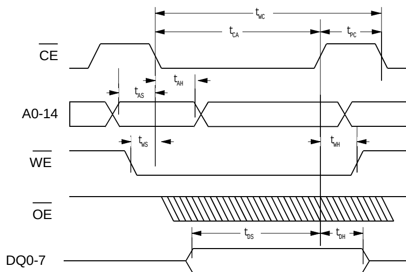
/CE-Controlled Write Cycle Timing
