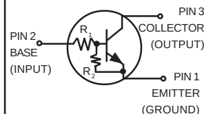
SC-59 CASE 318D, STYLE 1
