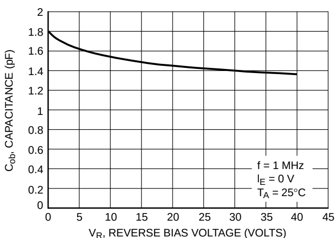
Figure 29. Output Capacitance
