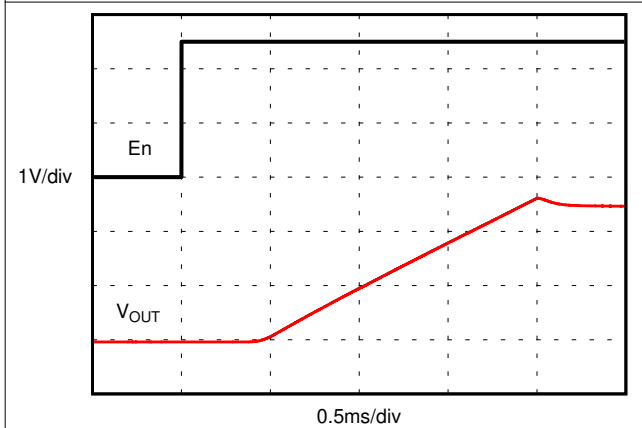
Figure 8-23. Turnon Time (Enable)
