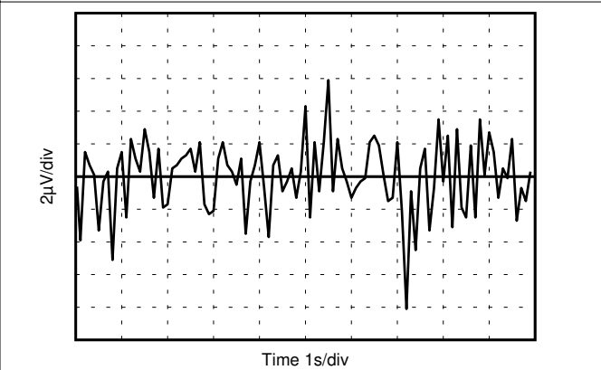
Figure 8-24. 0.1-Hz to 10-Hz Noise ( V_{REF} )
