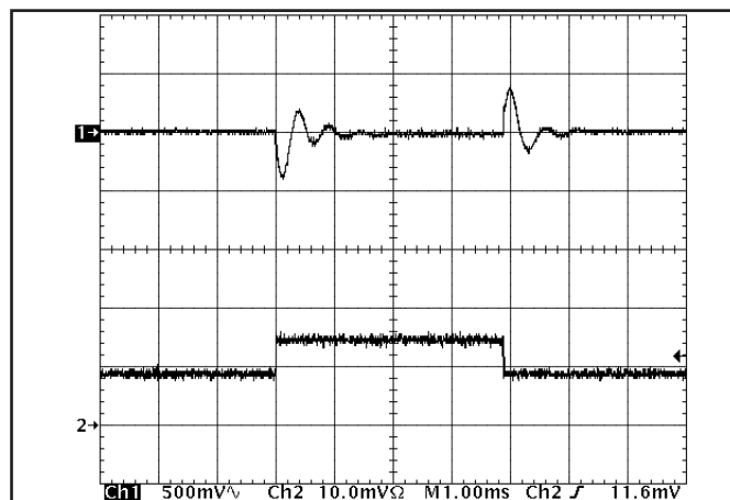
Figure 12: Output voltage response to step-change in load current (50%-75%-50% of I_{out(max)} ; dI/dt = 5\text{A}/\mu\text{s} ). Load cap: 480 \mu\text{F} , 15 m \Omega ESR tantalum cap and 1 \mu\text{F} ceramic cap. Top trace: V_{out} (500mV/div), Bottom trace: I_{out} (5A/div).
