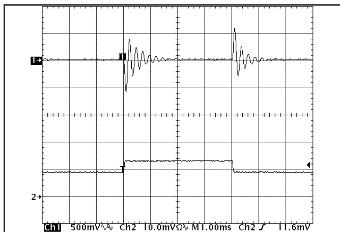
Figure 11: Output voltage response to step-change in load current (50%-75%-50% of I_{out(max)} ; dI/dt = 0.1\text{A}/\mu\text{s} ). Load cap: 15 \mu\text{F} , 450 m \Omega ESR tantalum cap and 1 \mu\text{F} ceramic cap. Top trace: V_{out} (500mV/div), Bottom trace: I_{out} (5A/div).
