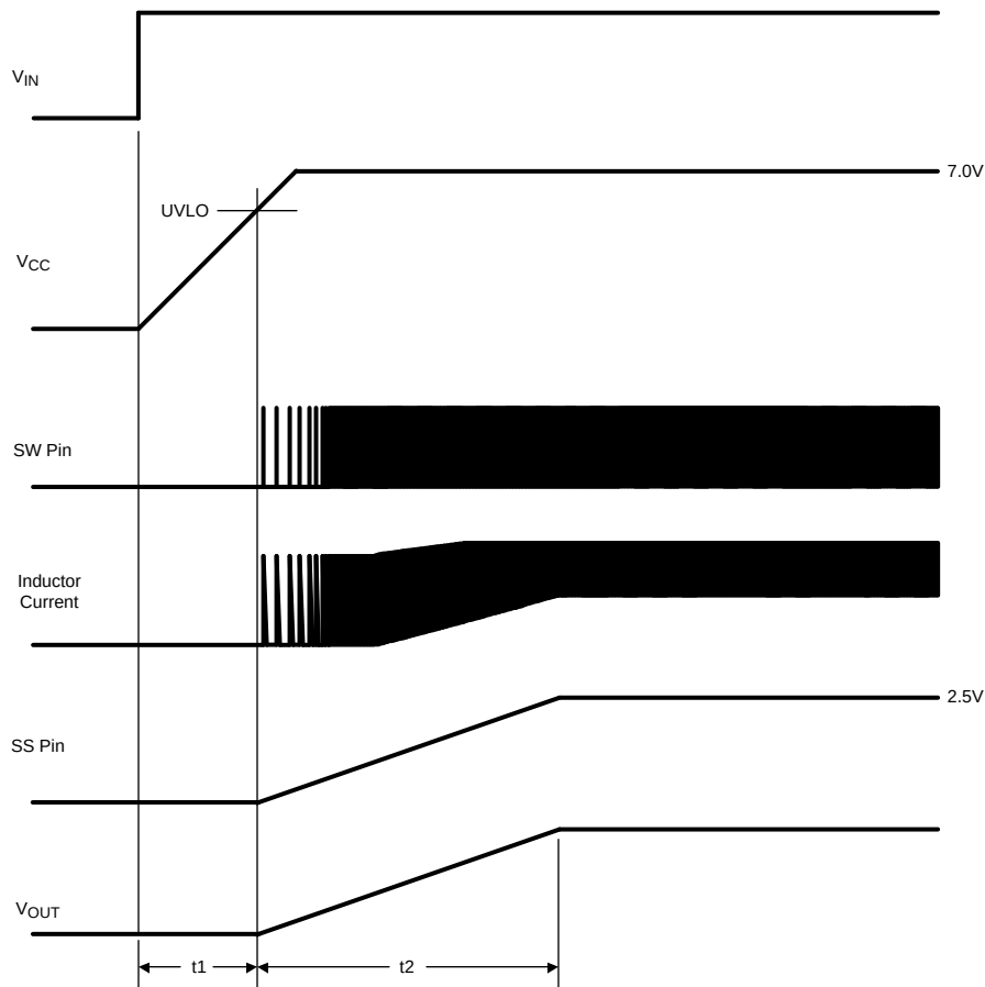
Figure 2. Startup Sequence
