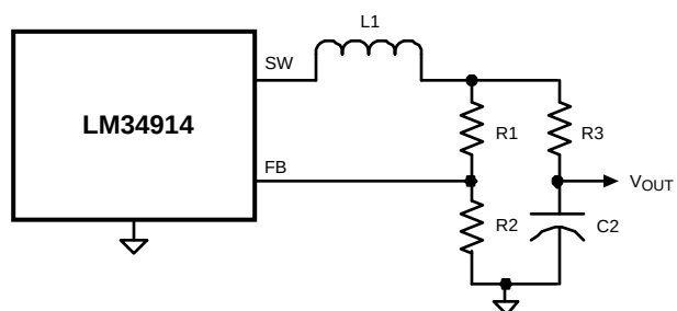
Figure 7. Alternate Minimum Output Ripple
