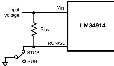
Figure 3. Shutdown Implementation
