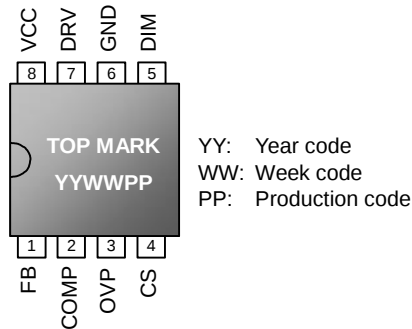
SOP-8 (TOP VIEW)
