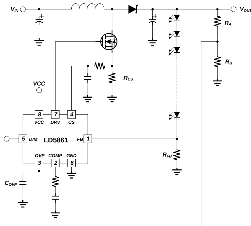
Fig. 1 Application circuit
