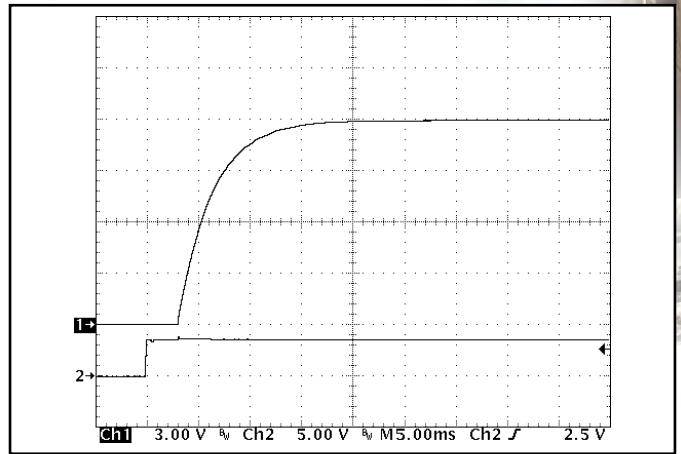
Figure 8: Turn-on transient at full resistive load and 3 mF output capacitance initiated by ENA1. Input voltage pre-applied. Ch 1: Vout (3V/div). Ch 2: ENA1 (5V/div).
