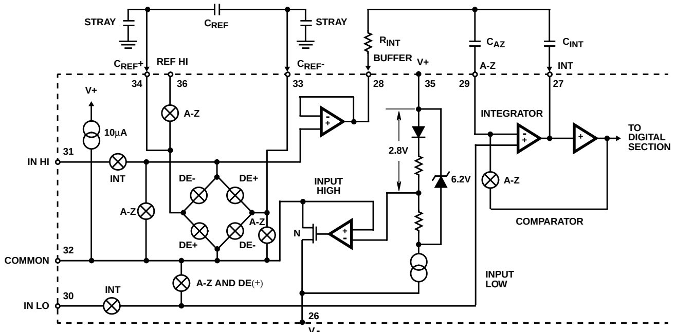
FIGURE 3. ANALOG SECTION OF ICL7116 AND ICL711
