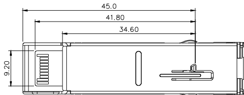
Bottom View
