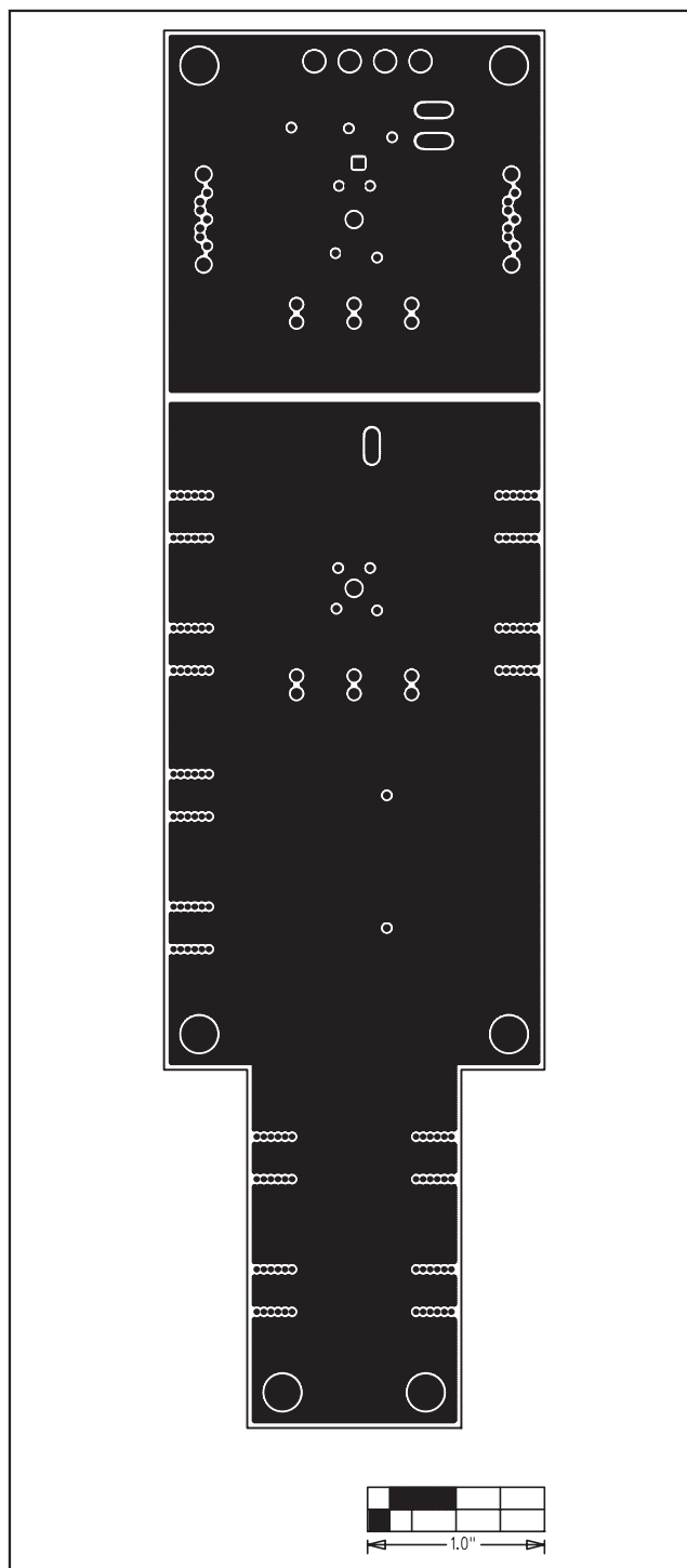
Figure 5. MAX4951 EV Kit PCB Layout—Inner Layer 3
