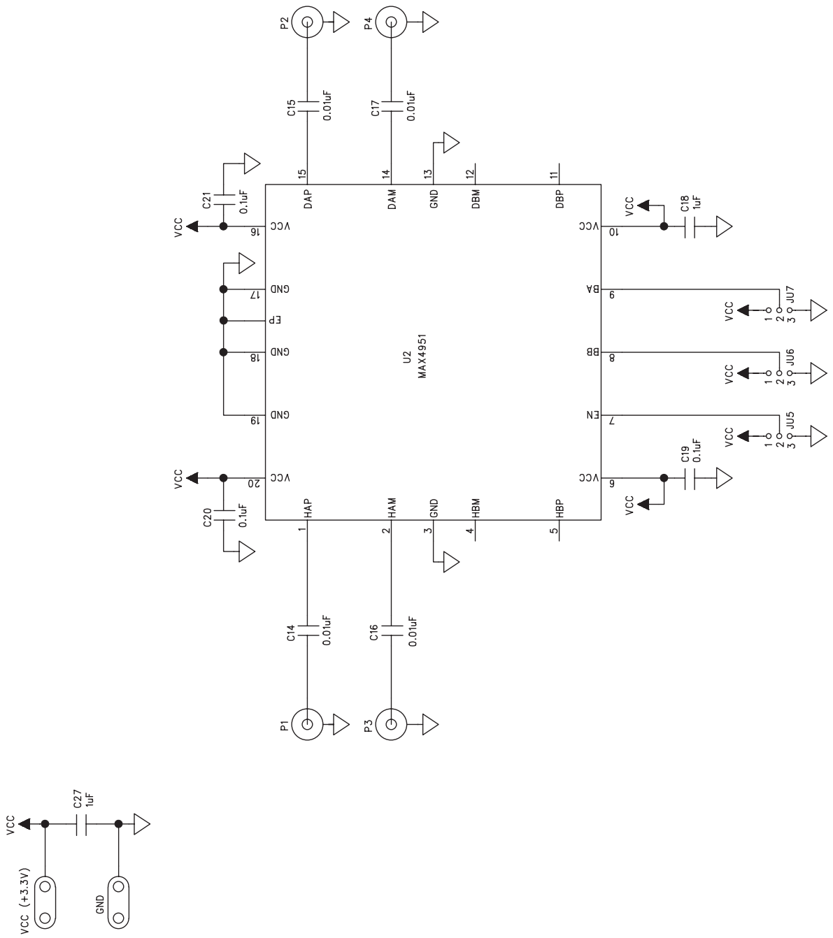
Figure 1b. MAX4951 EV Kit Schematic (Sheet 2 of 3)
