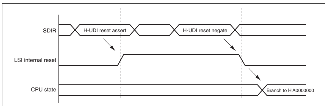
Figure 21.4 H-UDI Reset
