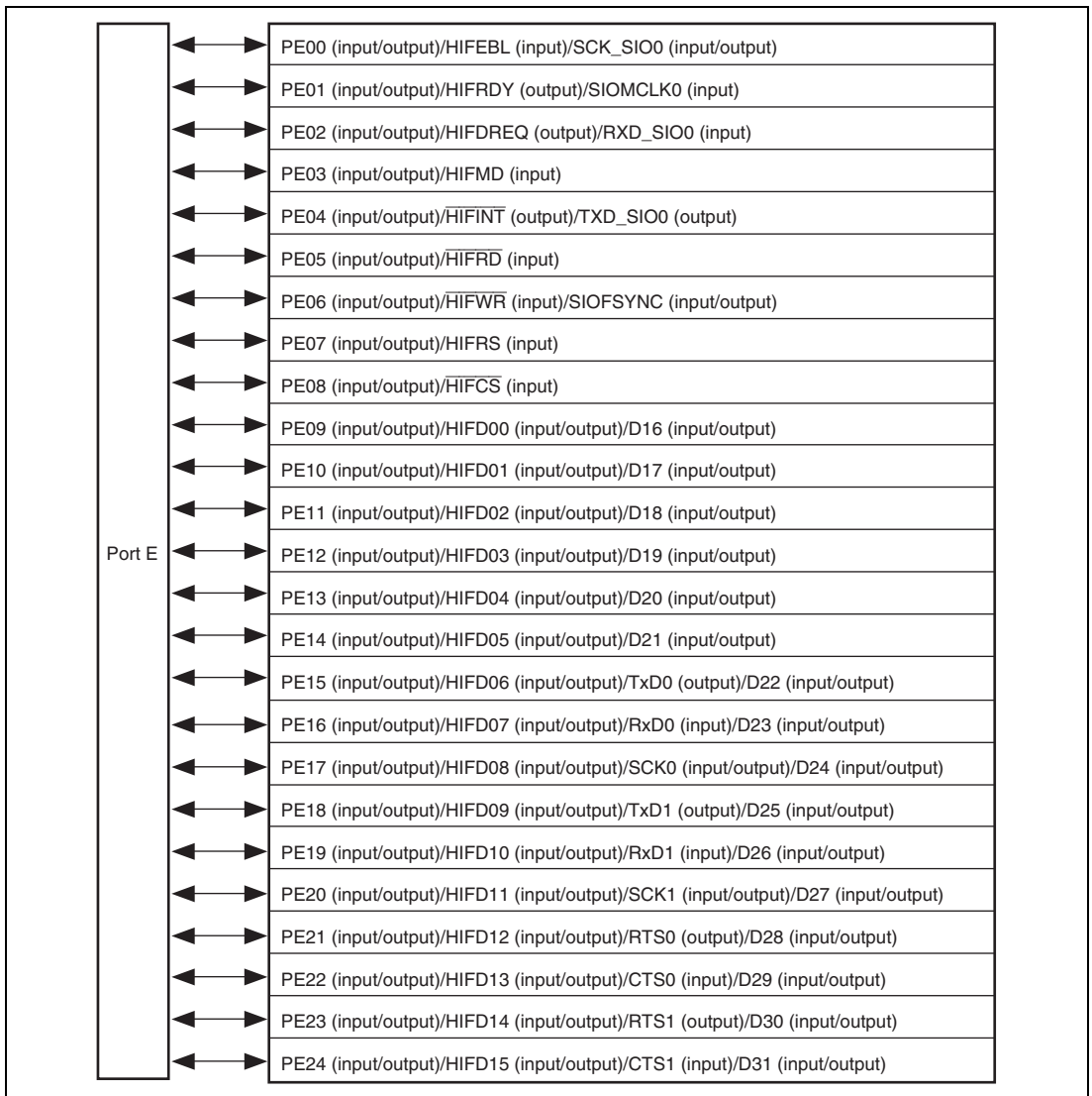
Figure 19.5 Port E
