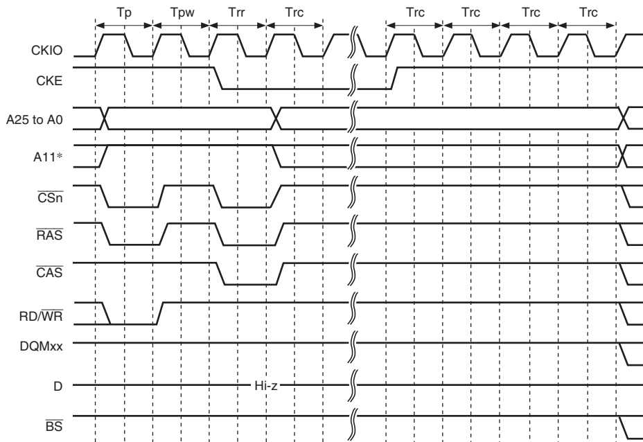
Figure 7.26 Self-Refreshing Timing
