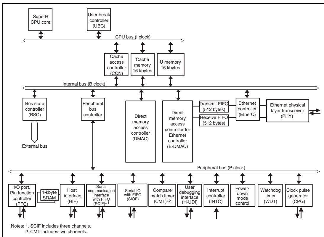
Figure 1.1 Block Diagram
