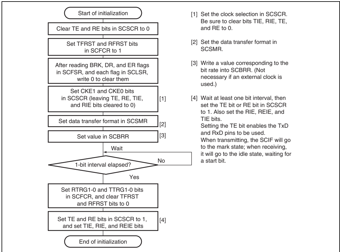
Figure 15.3 Sample Flowchart for SCIF Initialization
