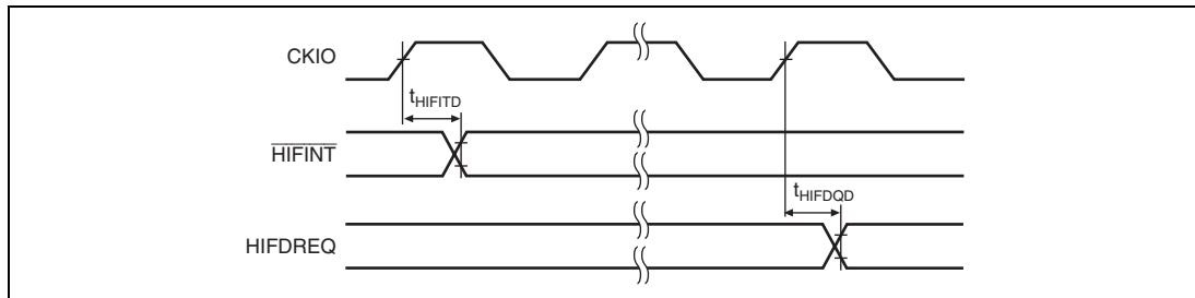
Figure 25.49 \overline{\text{HIFINT}} and HIFDREQ Timing
