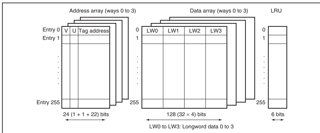
Figure 3.1 Cache Structure
