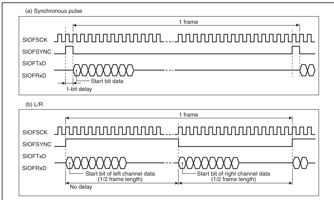
Figure 16.3 Serial Data Synchronization Timing
