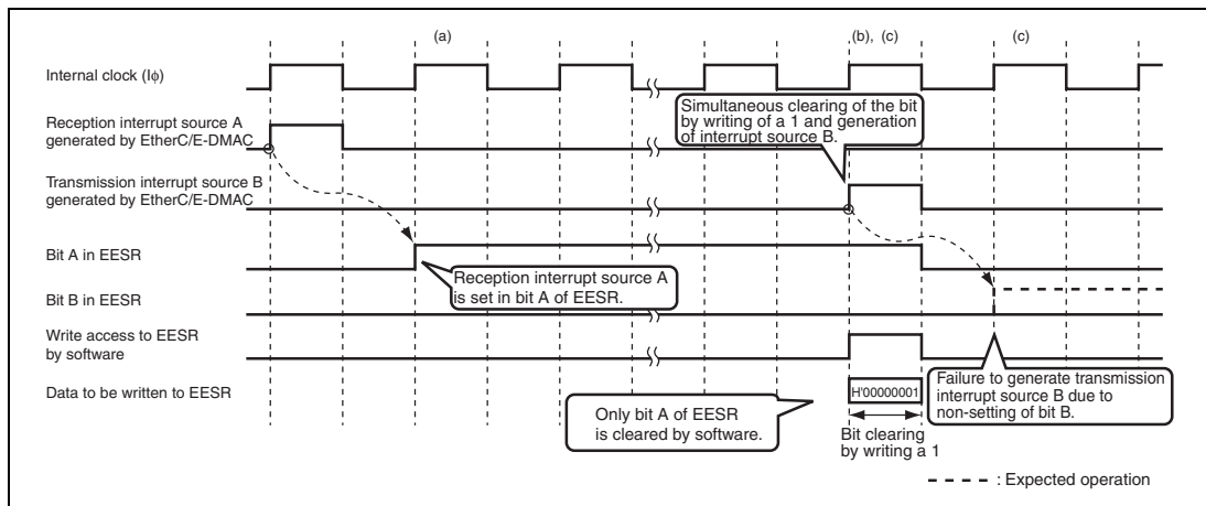
Figure 12.8 Timing of the Case where Setting of the Interrupt Source Bit in EESR by the E-DMAC Fails
