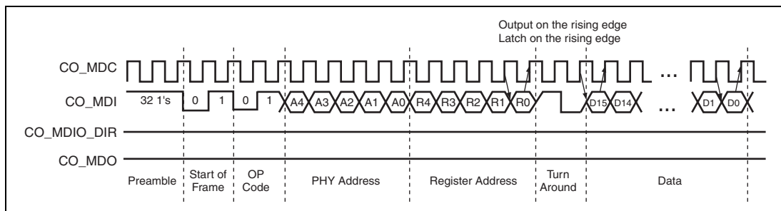
Figure 22.5 MDIO Timing and Frame Structure (WRITE Cycle)
