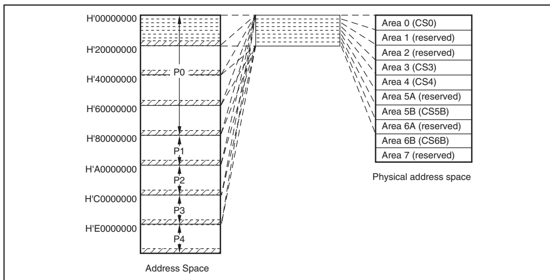
Figure 7.2 Address Space
