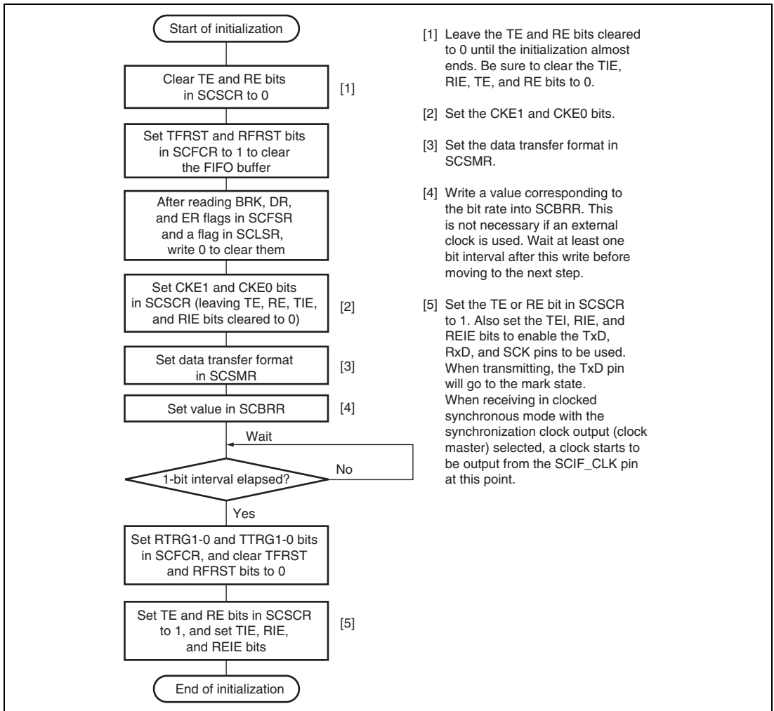
Figure 15.12 Sample Flowchart for SCIF Initialization
