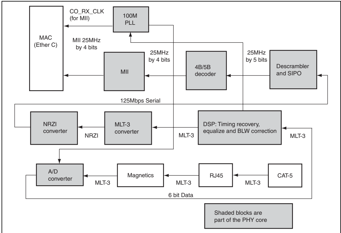
Figure 22.7 Receive Data Path
