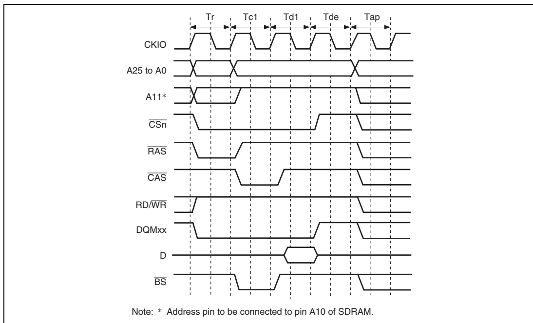
Figure 7.16 Basic Timing for Single Read (Auto Precharge)
