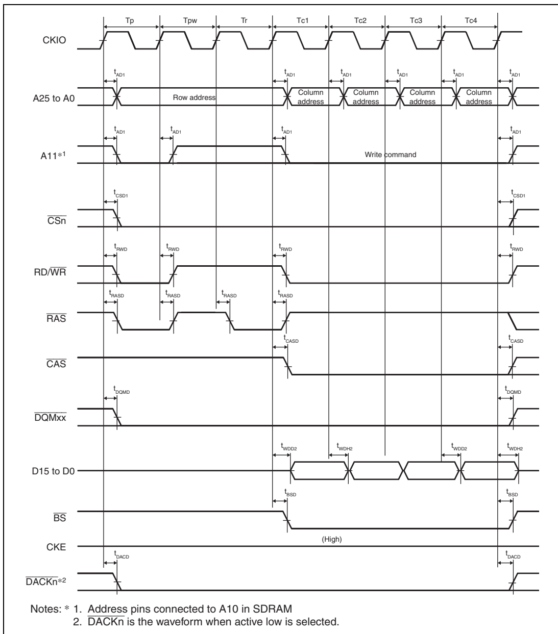
Figure 25.29 Synchronous DRAM Burst Write Bus Cycle (Single Write × 4) (Bank Active Mode: PRE + ACT + WRITE Commands, Different Row Addresses, WTRCD = 0 Cycle, TRWL = 0 Cycle)
