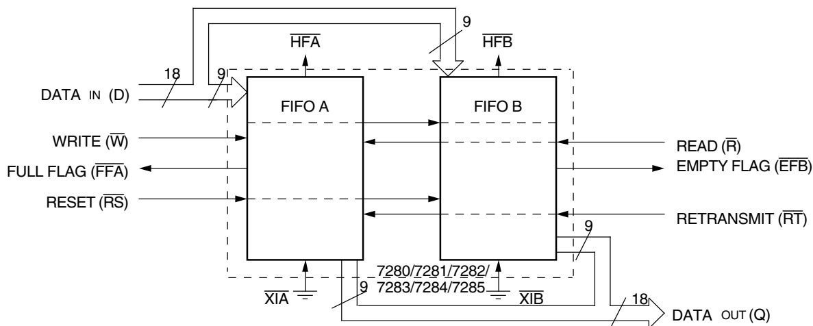
Figure 13. Block Diagram of 256 x 18, 512 x 18, 1,024 x 18, 2,048 x 18, 4,096 x 18, 8,192 x 18 FIFO Memory Used in Width Expansion Mode
