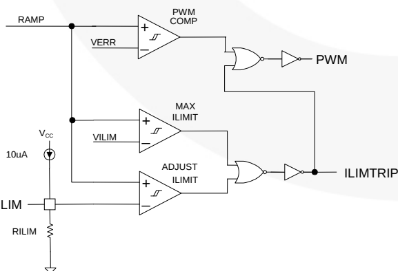
Figure 24. Current-Limit System Schematic
