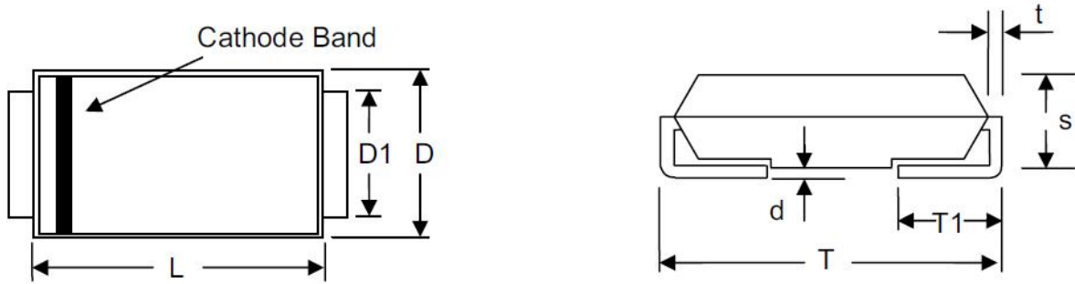
SMB/DO-214AA
