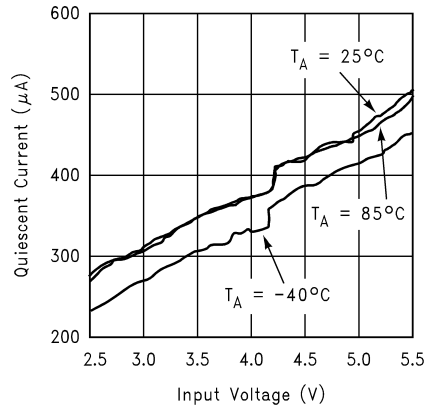
Operating Quiescent Current vs. V_{IN}
