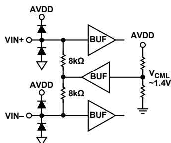
Figure 19. Analog Inputs ( V_{CML} \approx 1.4\text{ V} )
