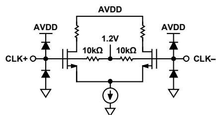
Figure 18. Clock Inputs
