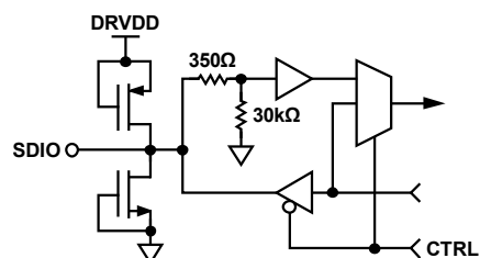
Figure 22. SDIO
