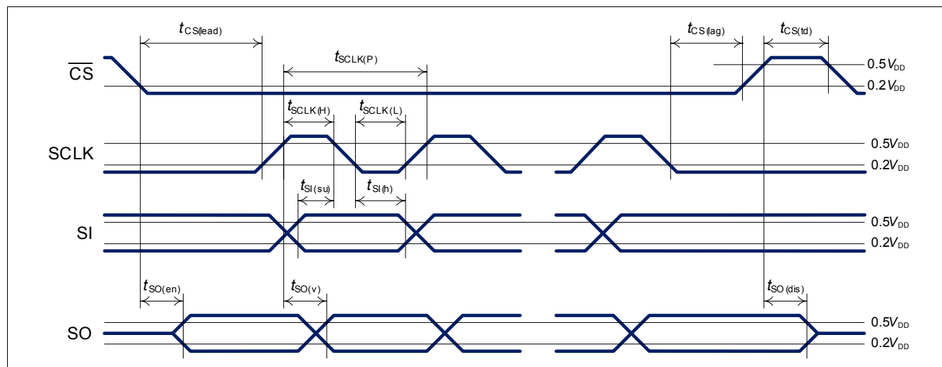
Figure 13 Timing Diagram
