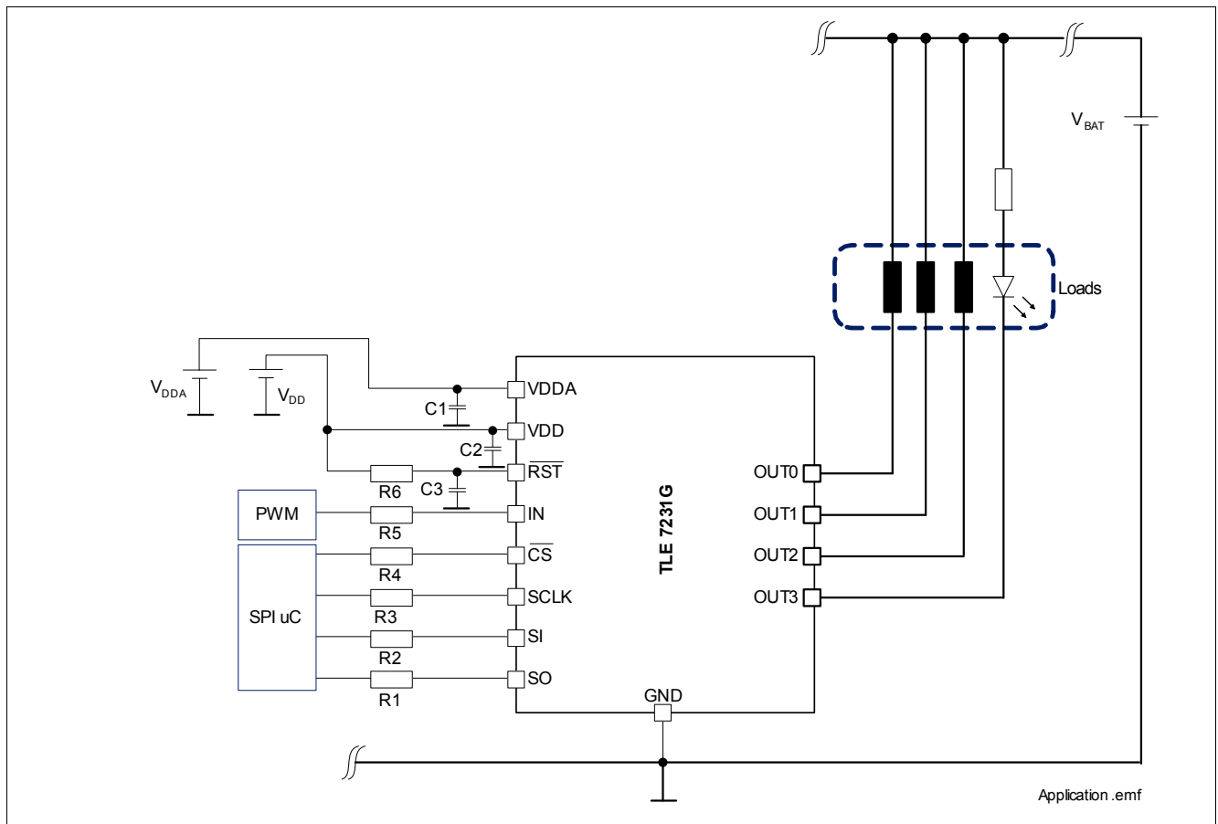
Figure 14 Application Diagram
