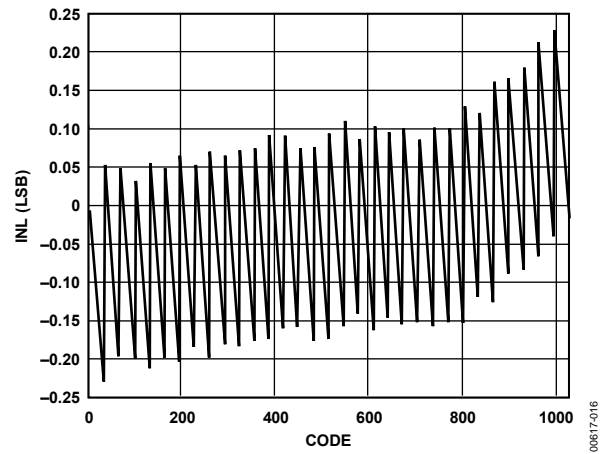
Figure 16. Typical INL
