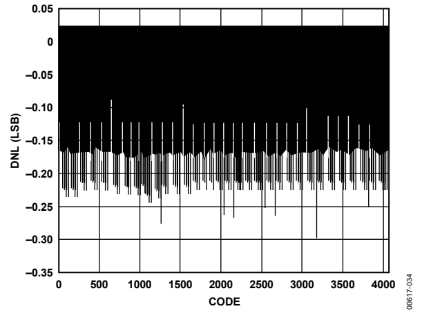
Figure 34. Typical DNL
