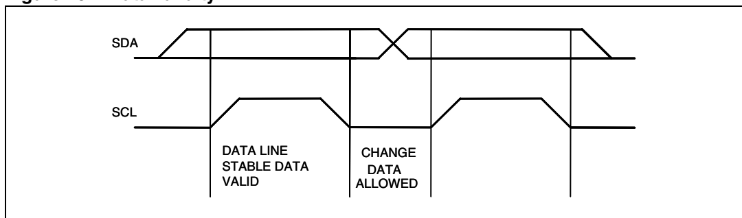
Figure 16. Data validity
