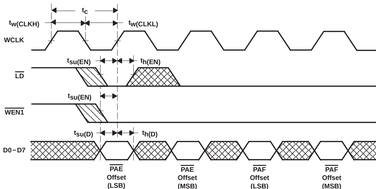
Figure 10. Write-Offset-Registers Timing
