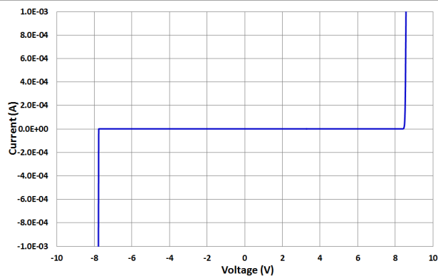
Figure 6-5. IV Curve
