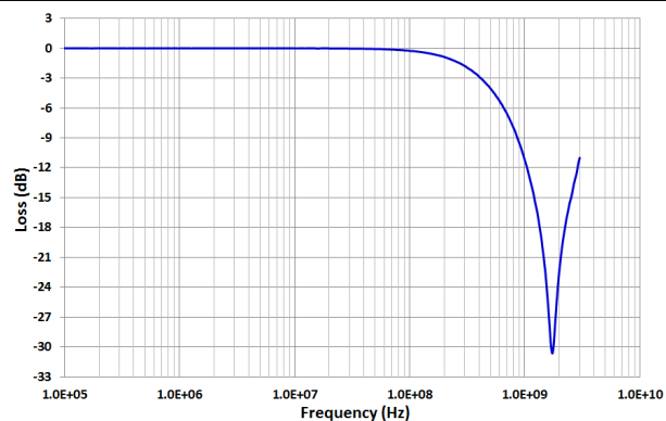
Figure 6-9. Insertion Loss
