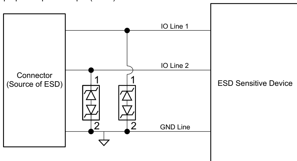
Application Schematic
