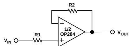
Figure 44. A Resistance in Series with an Input Limits Overvoltage Currents to Safe Values
