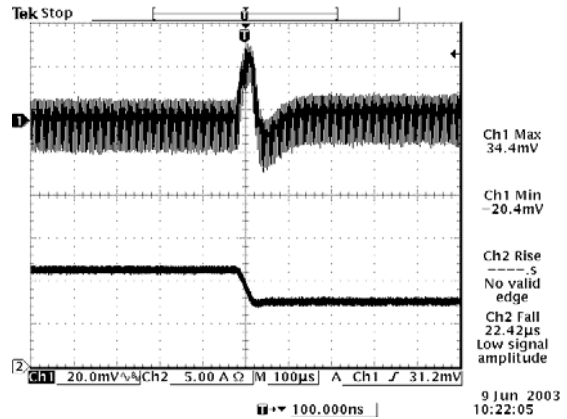
Transients 75% to 50% load, 1.5 Vdc Output
