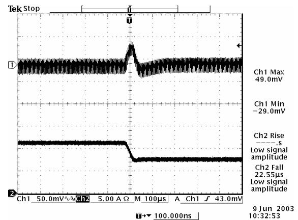
Transients 75% to 50% load, 2.5 Vdc Output
