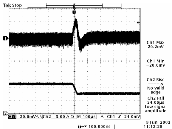
Transients 75% to 50% load, 1.2 Vdc Output
