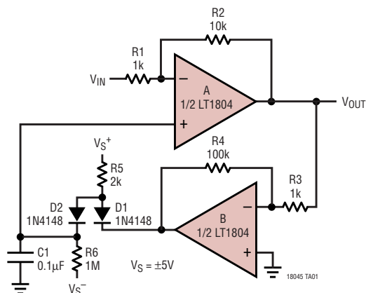
Inverting DC Restore
