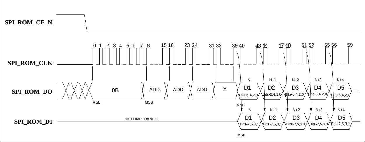
FIGURE 3-5: SPI ROM DUAL HI-SPEED READ SEQUENCE
