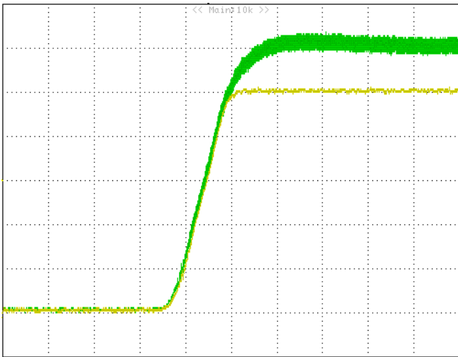
Figure 23: Tracking function, V_{tracking}=6V , V_{out}= 5.0V , full load Yellow : V_{OUT} , (1V/div), Green: Tracking, (1V/div), 500 \mu S/div
