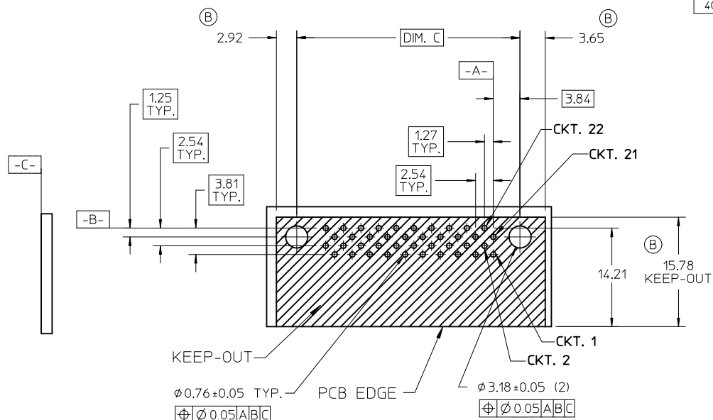
RECOMMENDED PCB LAYOUT SHOWN FROM COMPONENT SIDE
