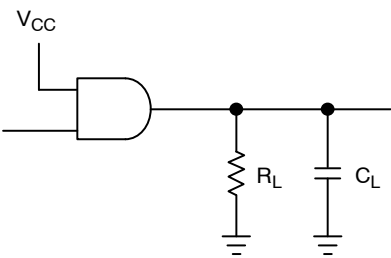
A 1-MHz square input wave is recommended for propagation delay tests.
